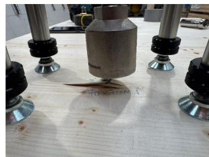
Figure 34 Load pull out close up
