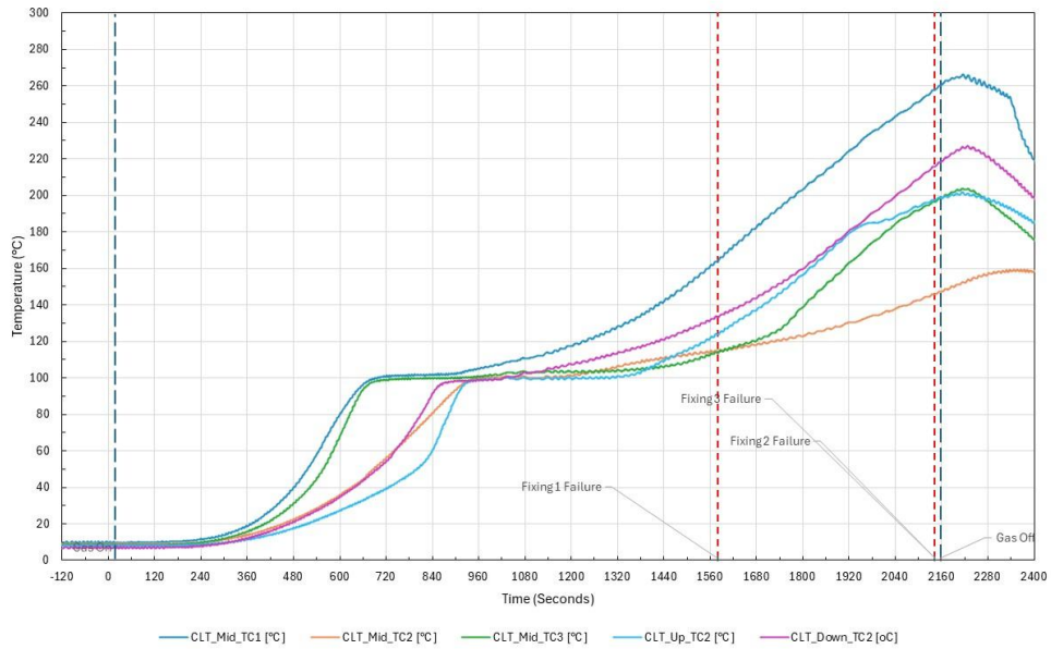
Coach Screw Pilot Hole study - CLT temperatures 20mm above original fire surface
