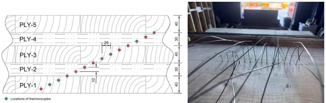
Figure 28 Position of thermocouples within the CLT for detailed thermal analysis
