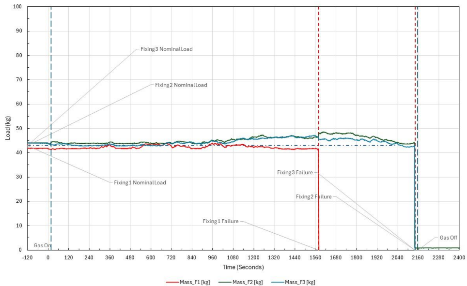
Coach Screw Pilot Hole study - Load on fixings
